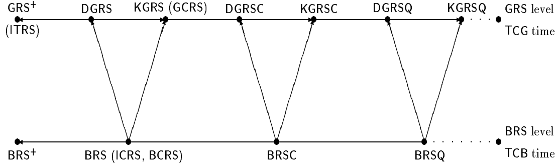
Fig. 1. Barycentric and Geocentric Reference Systems (RSs) B — barycentric, G — geocentric, C — ecliptical, Q — equatorial, D — dynamical, K — kinematical, + — rotating (Brumberg et al., 1996); ICRS — International Celestial RS, ITRS — International Terrestrial RS (IERS); BCRS — Barycentric Celestial RS, GCRS — Geocentric Celestial RS (IAU, 2001)
