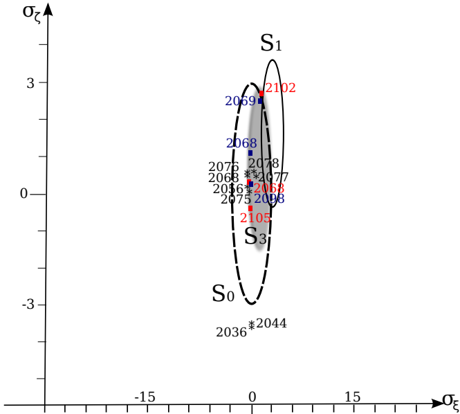
Fig. 1. 2029-b-plane of Apophis. The dotted 3\sigma ellipse is computed using solution S_0 . The solid 3\sigma ellipse is computed using solution S_1 and the blurred one with solution S_3 . For completeness, the center of primary ( \star ) and secondary keyholes leading to collision at ascending node ( \blacksquare ) and descending node ( \blacksquare ) are also represented. The figure is centered on the dotted ellipse and axis are expressed in sigma units of the S_0 solution.
