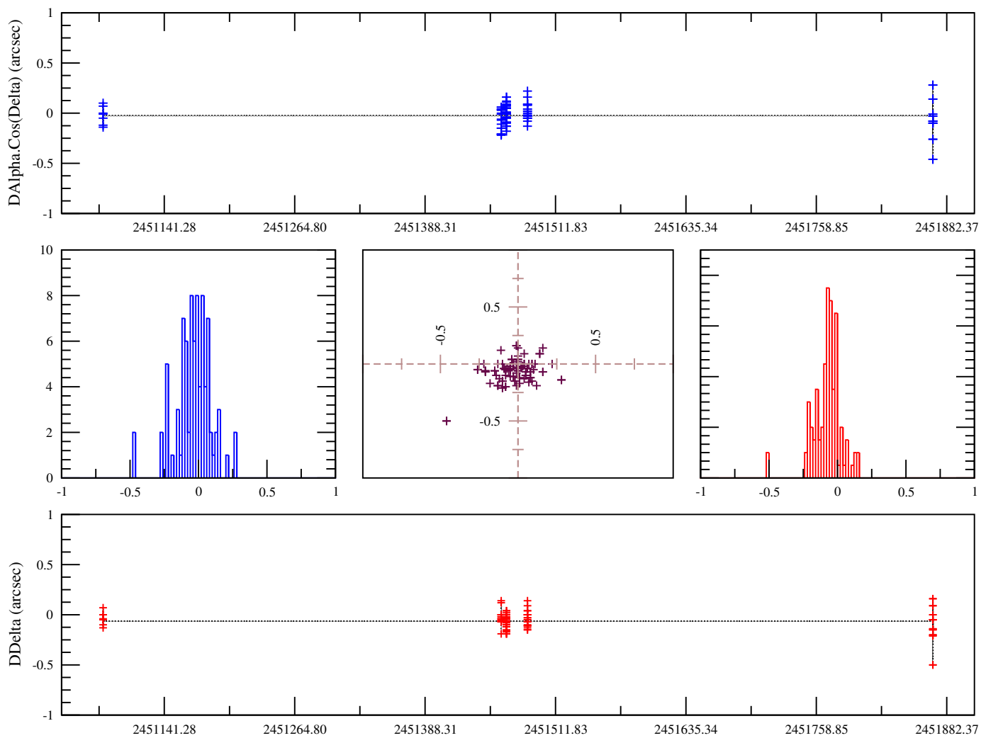
Observations Kulyk-Ledovskaya, 1998-2000, Pik Terskol, Ukraine. [UAI=B18] Satellite Amalthée - JPL Ephemeris
